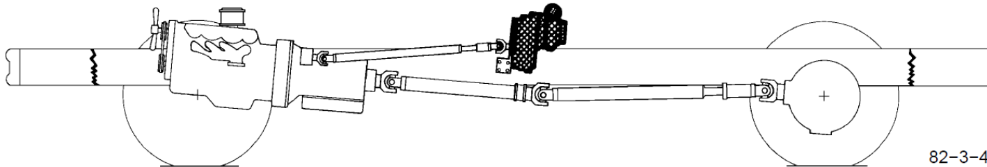
PTO Mounting
